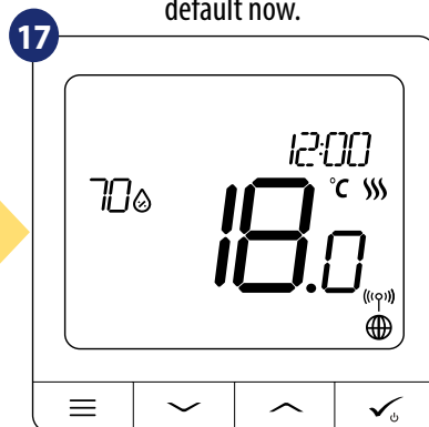
After that thermostat will display main screen. Congratulations! You successfully configured SQ610 Quantum thermostat as a wired device.
